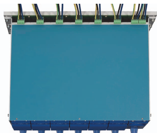
19" Rack Unit type PSS1250-HS-7-0/1/2/3/4-D Top view with cover
