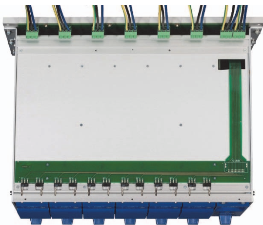
19" Rack Unit type PSS1250-HS-7-0/1/2/3/4-D Top view without cover
