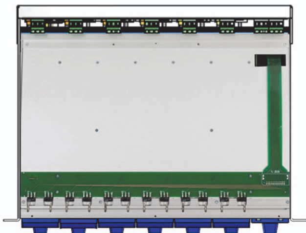
19" Rack Unit type PSS1250-HS-7-5/6/7/8/9-D Top view without cover
